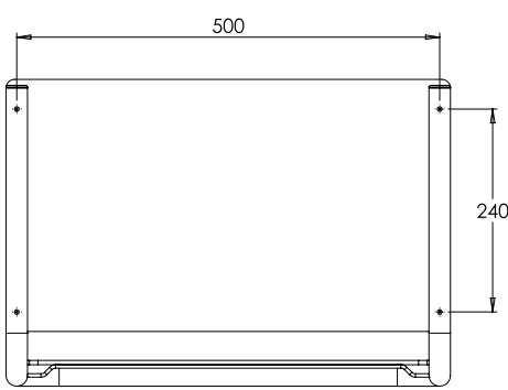
Wall fixing locations
